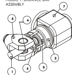
FIGURE 1: BALANCE BAR ASSEMBLY
