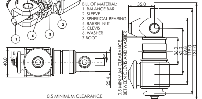
FIGURE 3: MAIN DIMENSIONS
