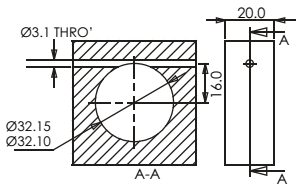
FIGURE 3: MAIN DIMENSIONS
